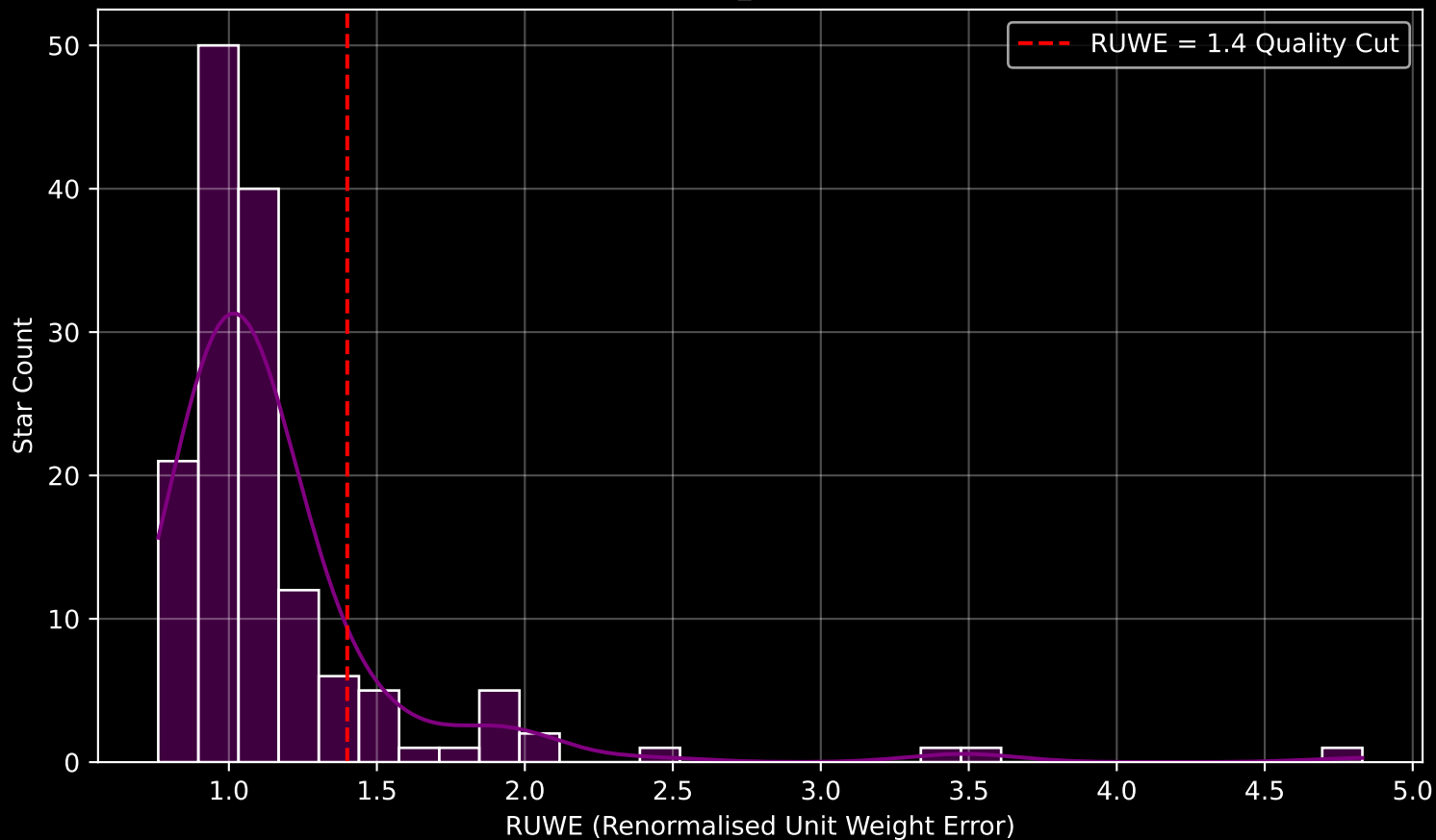
GAPOGEE DR17 Field [274-23-O_TESS] RUWE Distribution (n= 147)
