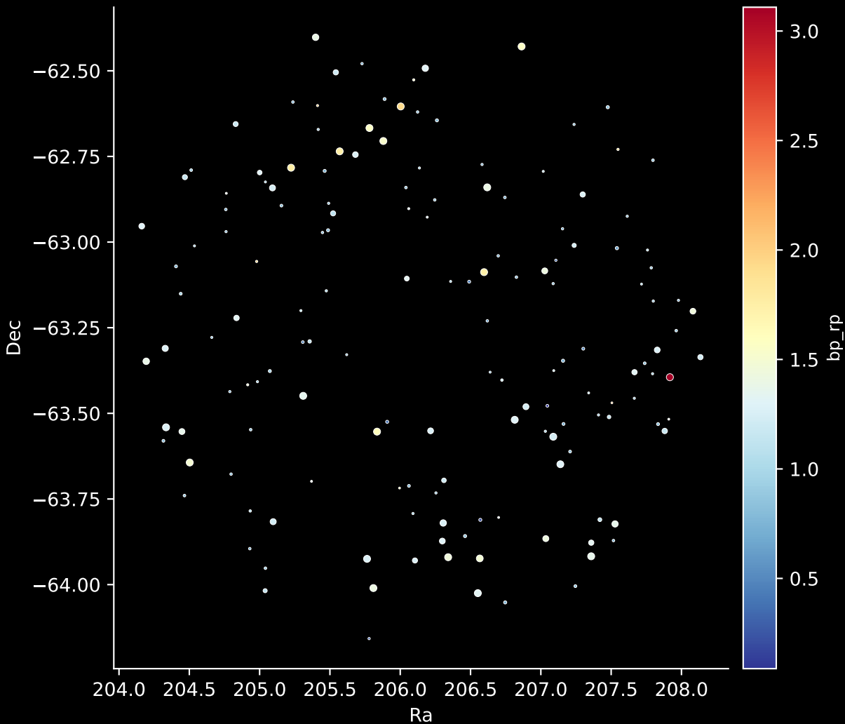
APOGEE DR17 Field: [274-23-O_TESS] Stars: 155
