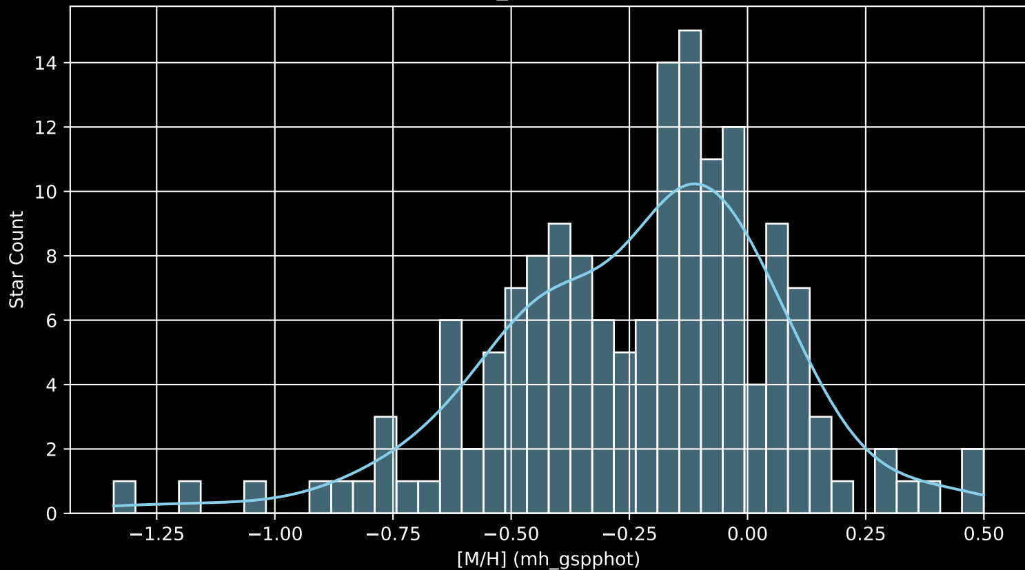
APOGEE DR17 Field: [274-23-O_TESS [M/H] (mh_gspphot) (n= 155)
