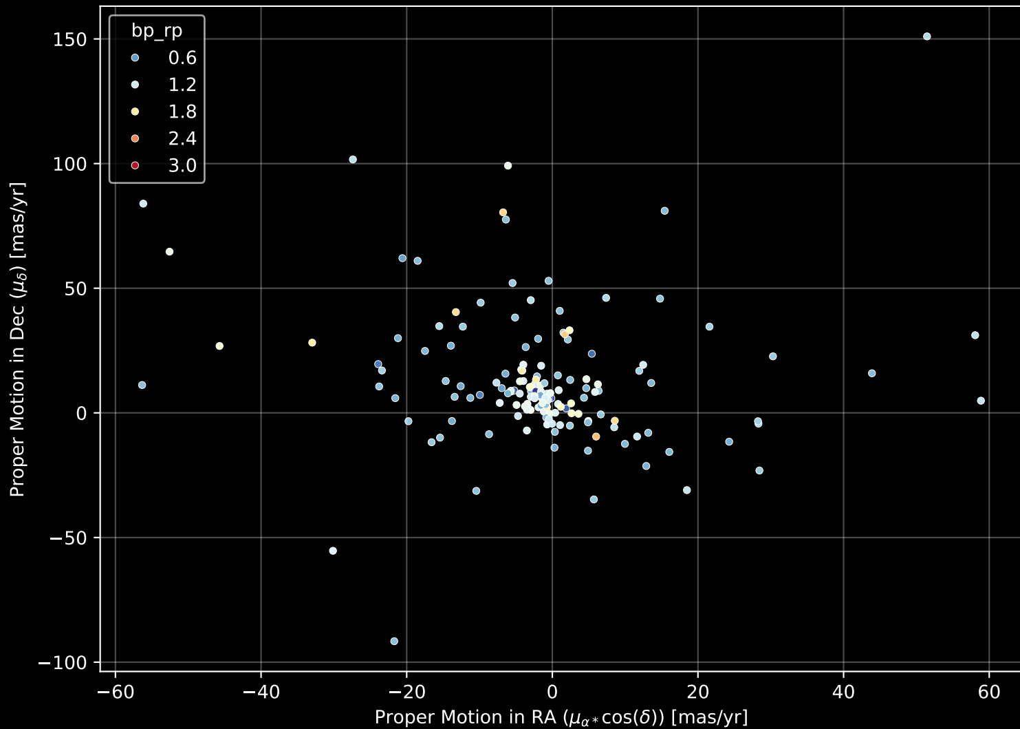
APOGEE DR17 Field: [274-23-O_TESS] Proper Motion Diagram (n= 155)
