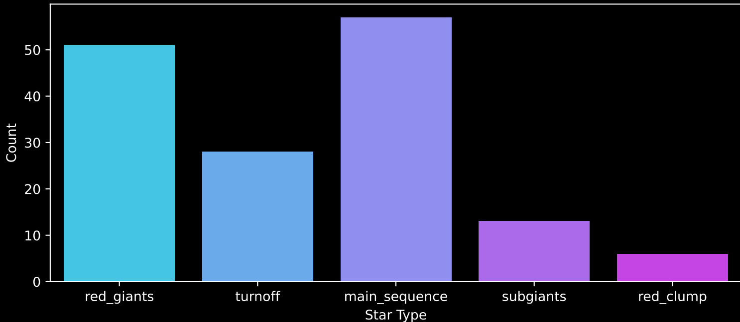
APOGEE DR17 Field: [274-23-O_TESS] Count plot of Star Type
