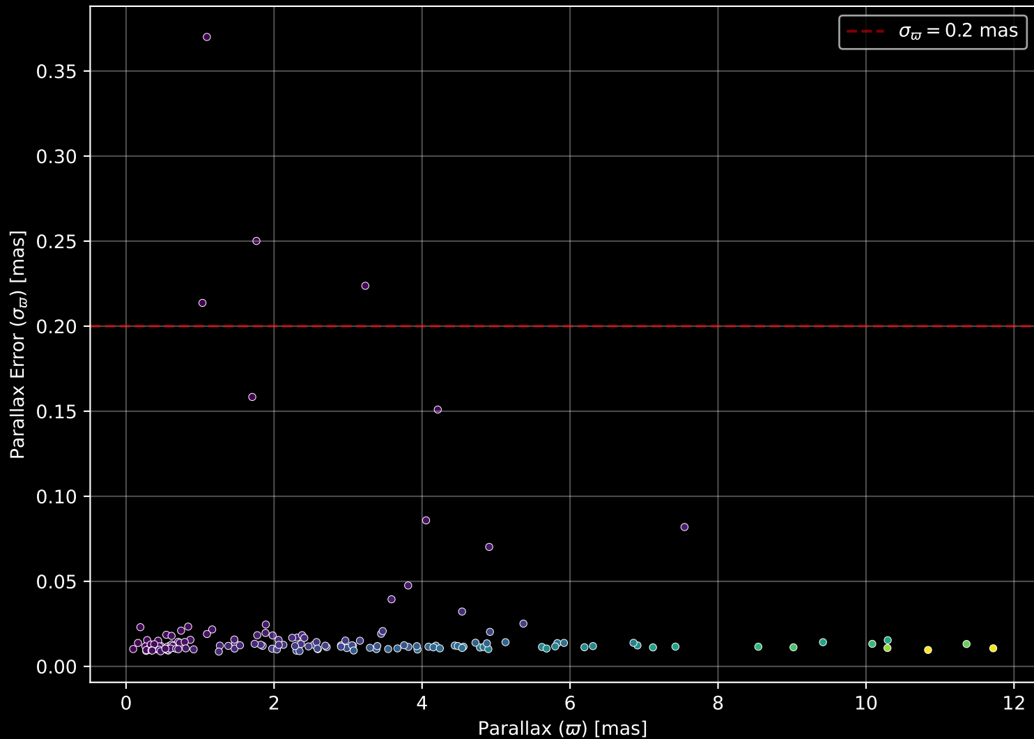
APOGEE DR17 Field: [274-23-O_TESS] Parallax Quality (n= 155)
