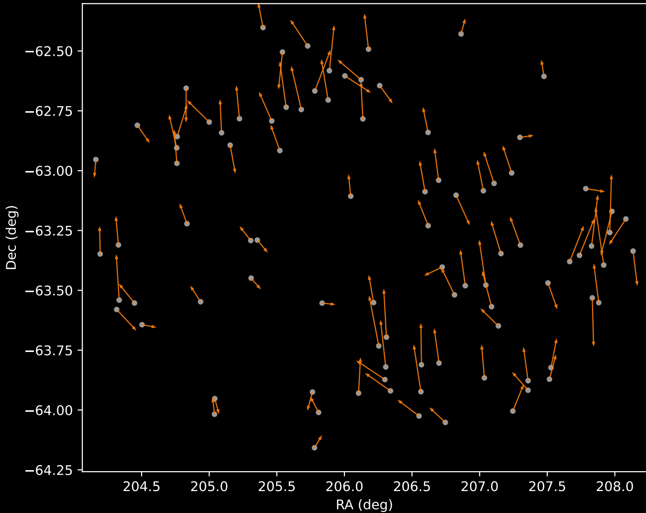
APOGEE DR17 Cluster 2 Proper Motion Vectors (n=92)
